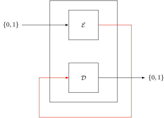
Figure 4: Sequential composition
